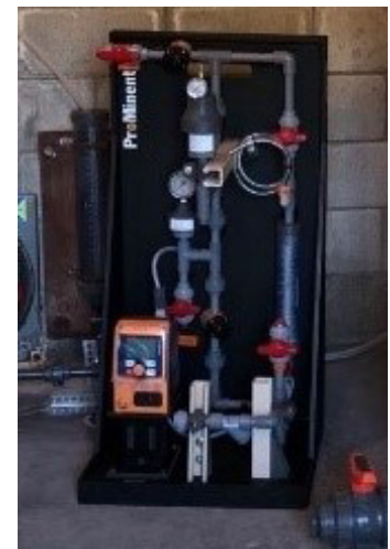
Pump Skid
